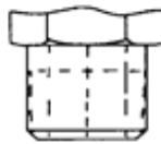
DIN 3852 Form C: Sealing by means of tapered thread. Female thread must be tapered to achieve rated operating pressure.
